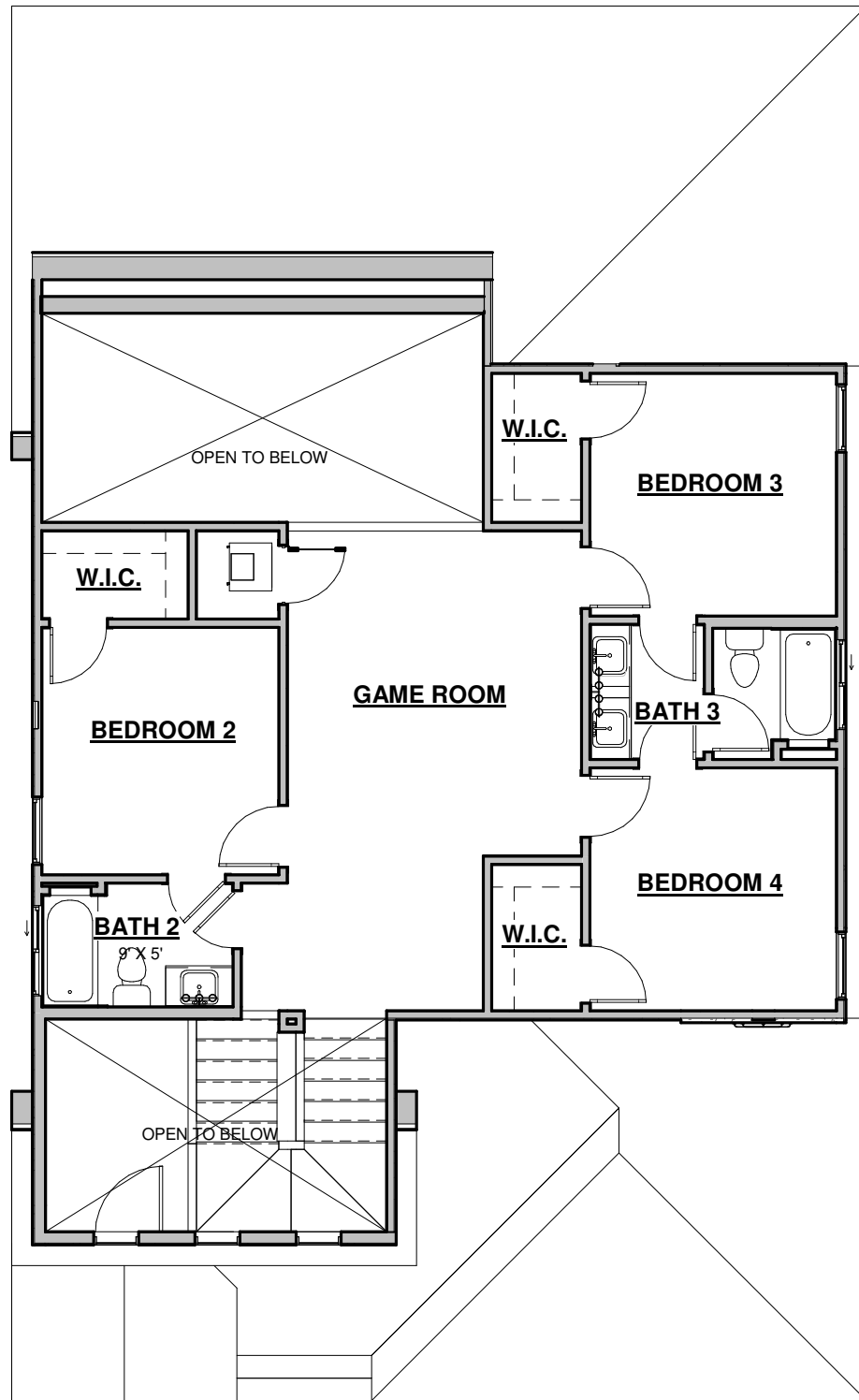
② SECOND FLOOR DIAGRAM NOT TO SCALE
