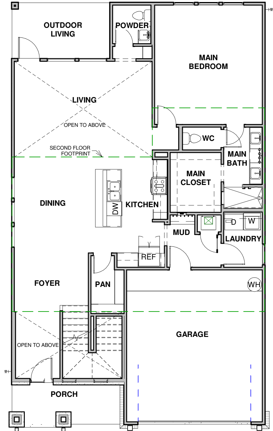
① FIRST FLOOR DIAGRAM NOT TO SCALE
