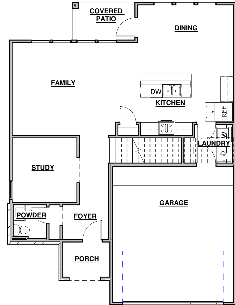
① FIRST FLOOR DIAGRAM PLAN NOT TO SCALE
